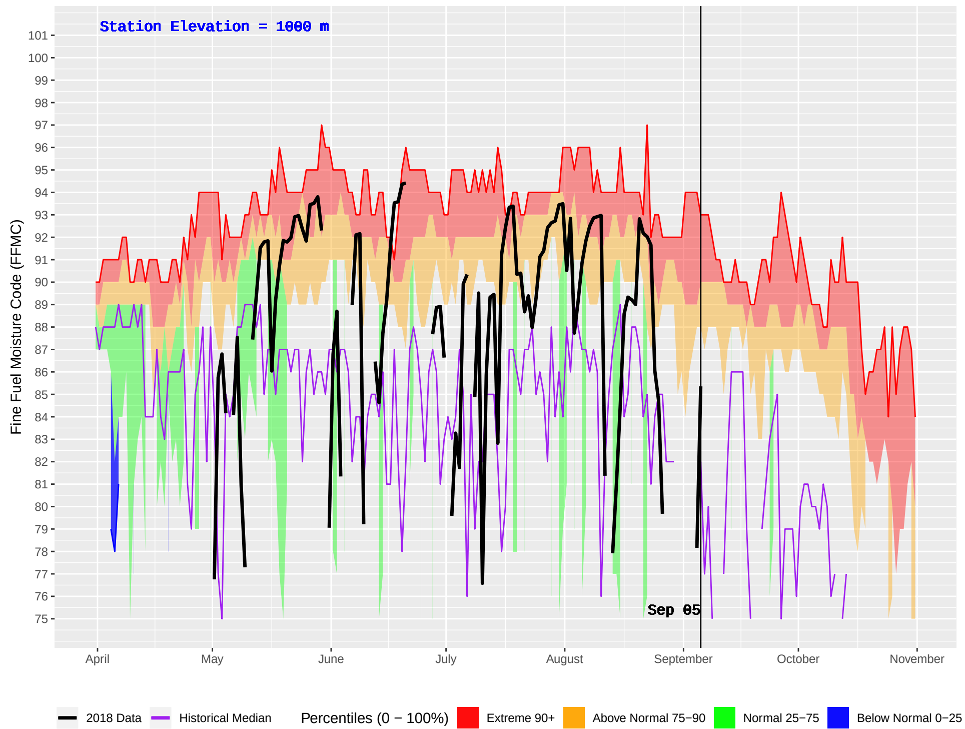
SUCCOUR CREEK (374) : Historical (1986–2016) and Current (2018) Daily Fine Fuel Moisture Code (FFMC)
