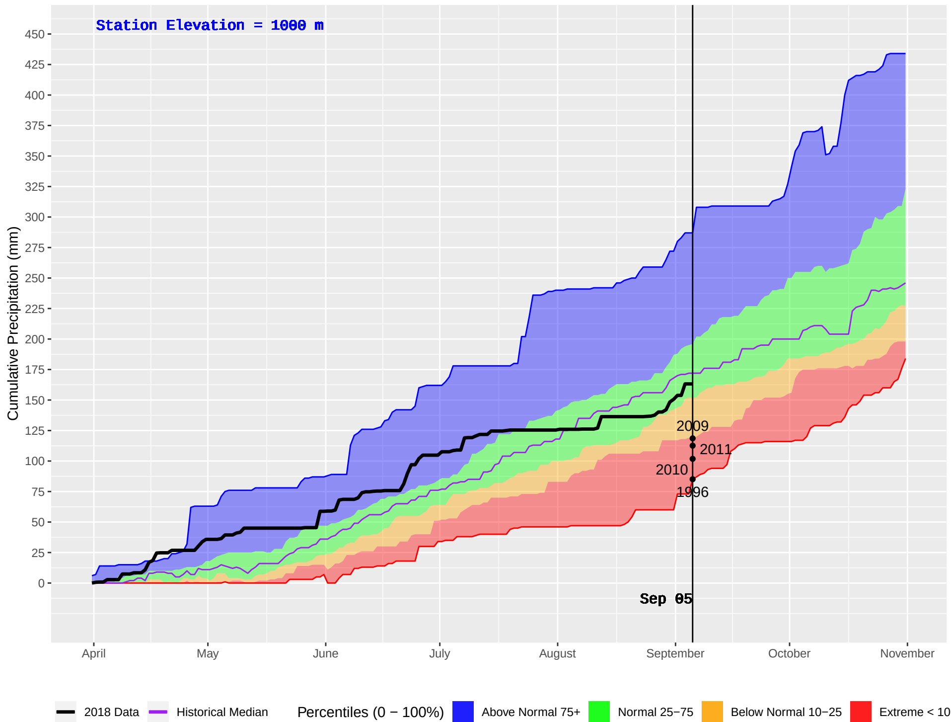
SUCCOUR CREEK (374) : Historical (1986–2016) and Current (2018) Daily Cumulative Precipitation
