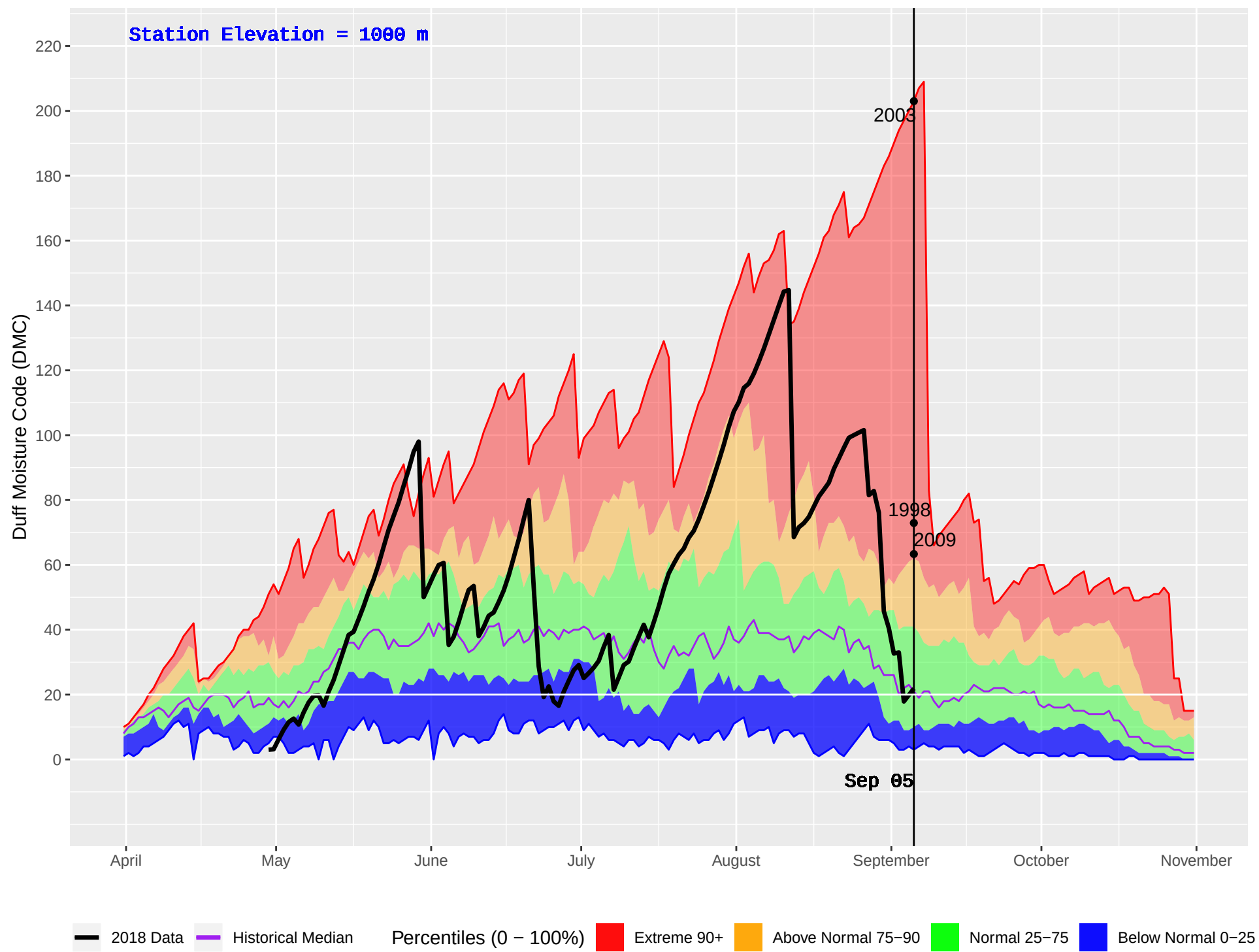
SUCCOUR CREEK (374) : Historical (1986–2016) and Current (2018) Daily Duff Moisture Code (DMC)
